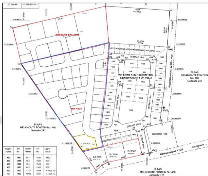
Figure 2: Site Development Plan - Snap
